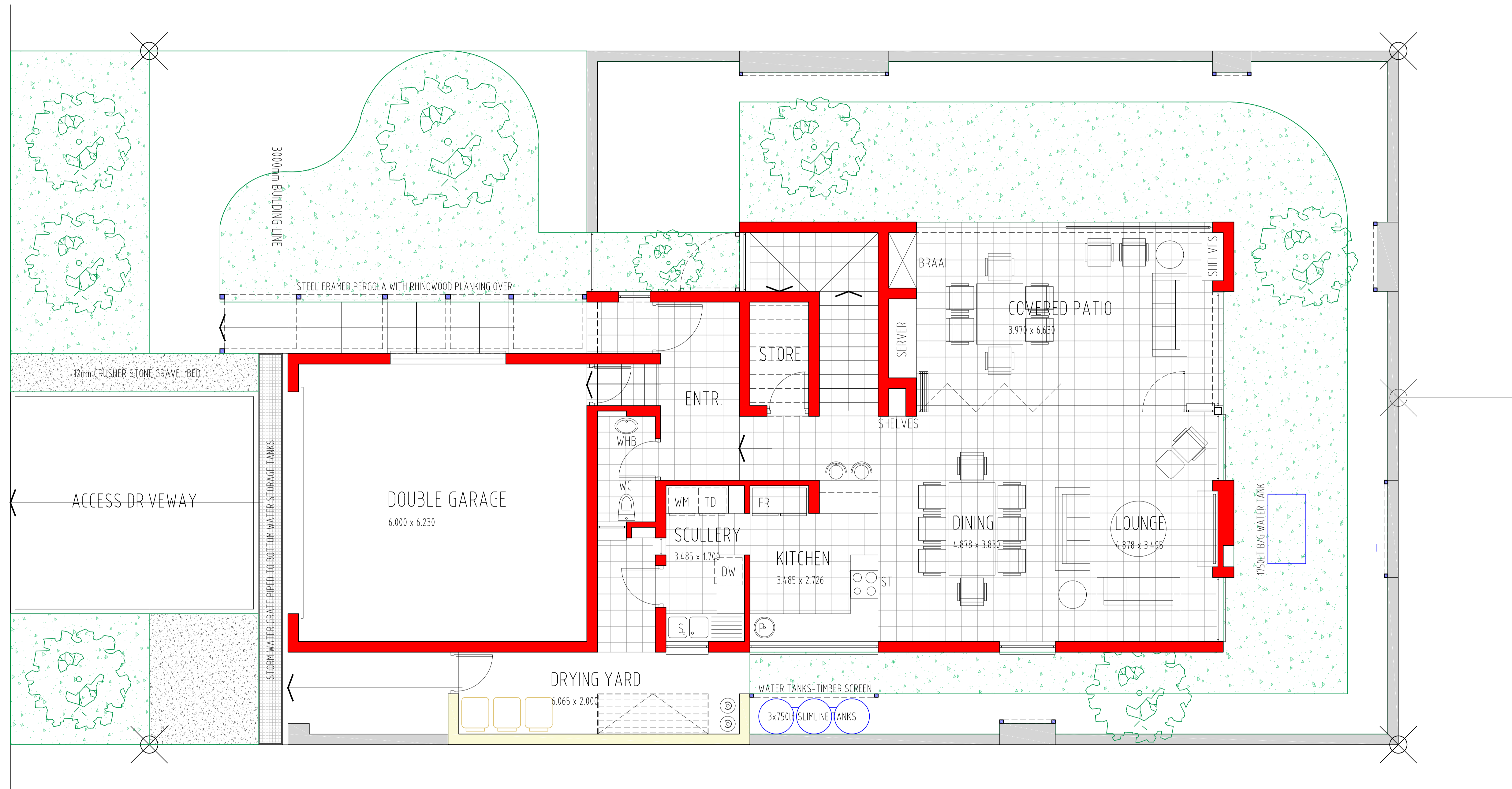
GROUND FLOOR
